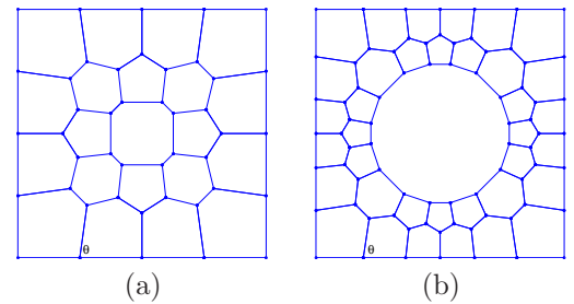
Figure 4: (a) 21-piece partition achieving \gamma = 1.32348 . Here \theta = 82.16^\circ . (b) 37-piece partition achieving \gamma = 1.31539 . Here \theta = 81.41^\circ .
