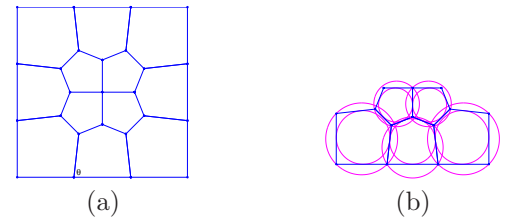
Figure 3: 12-piece partition achieving \gamma = 1.33964 (a) Overall design. Here \theta = 89.62^\circ . (b) Details of critical indisks and circumcircles.
